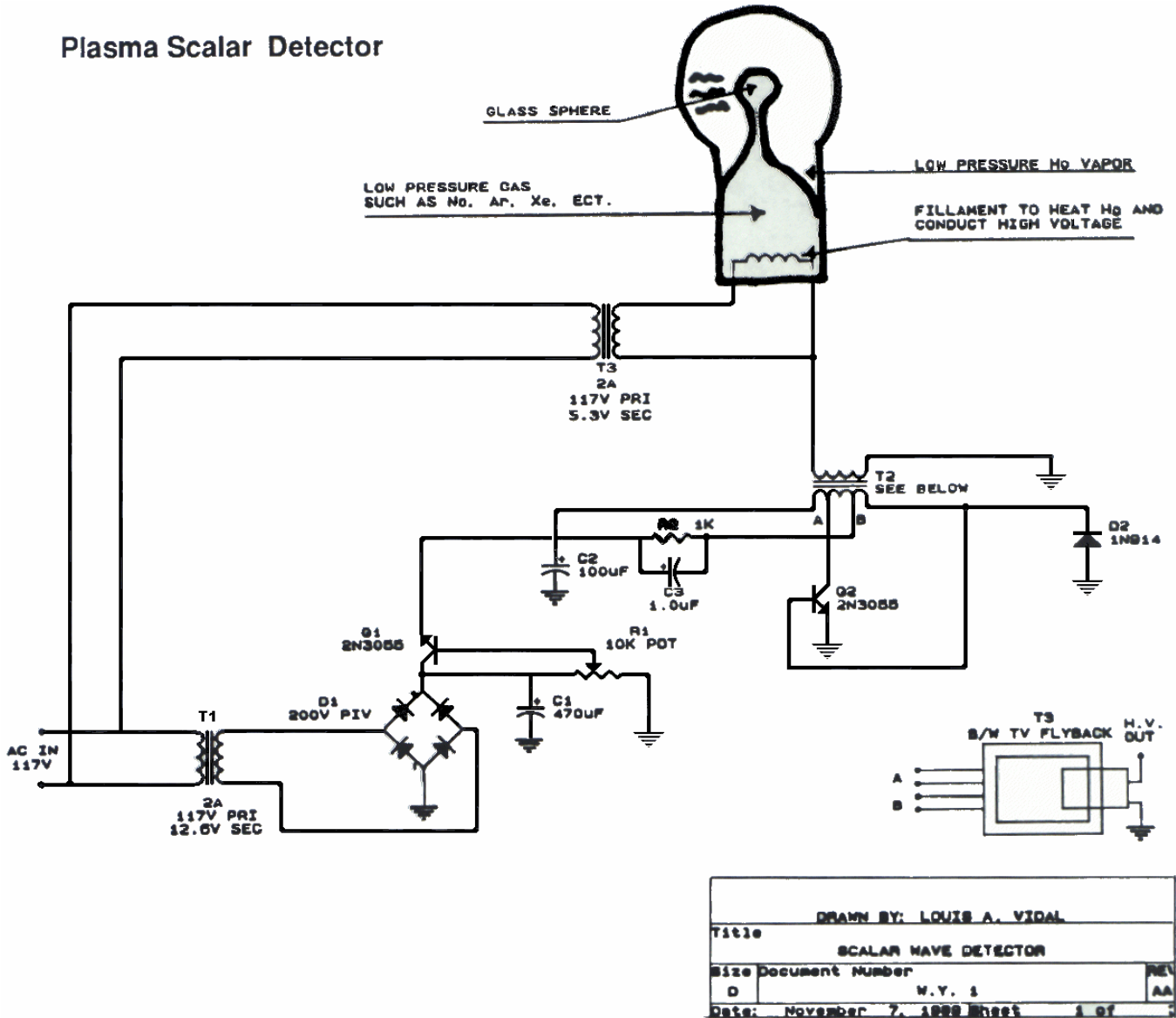
Figure 6. Plasma Scalar Detector
