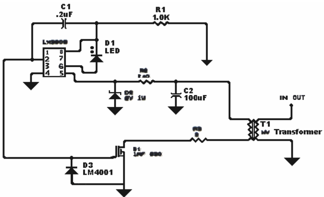
Figure 7. Power Supply
