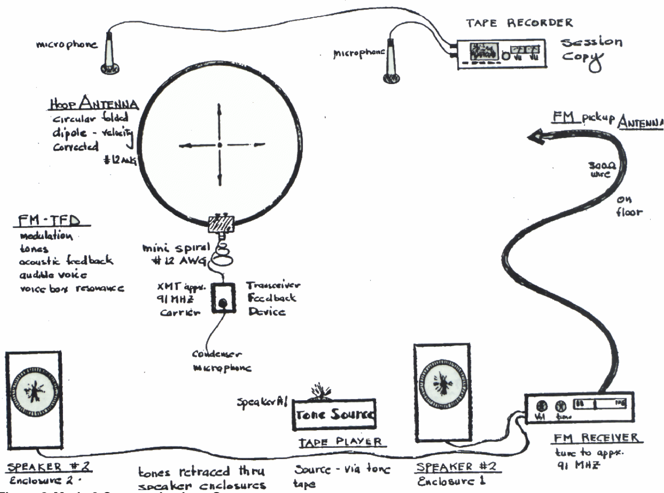
Figure 3. Mode 2 Communications Setup
